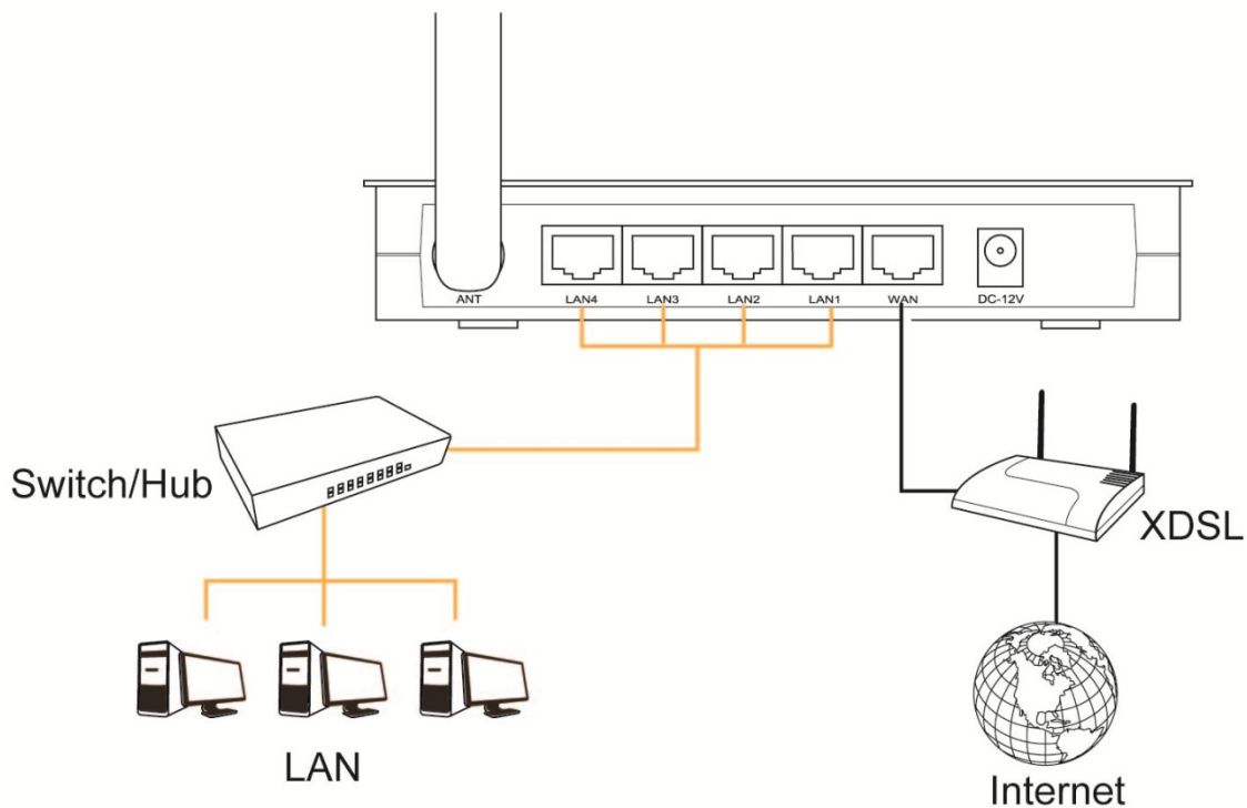
Figure 2-1 Hardware Installation of the AIP-W515H
